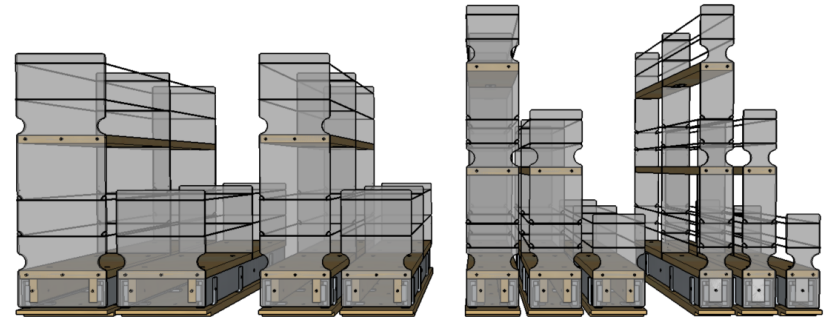
5x2x22 5x1x22 4x2x22 4x1x22 3x3x22 3x2x22 3x1x22 2x3x22 2x2x22 2x1x22 5.7" wide 16.52" tall 8" tall 22" deep 4.58" wide 16.52" tall 8" tall 22" deep 3.45" wide 19.52" tall 13" tall 6.52" tall 22" deep 2.25" wide 19.52" tall 13" tall 6.52" tall 22" deep
